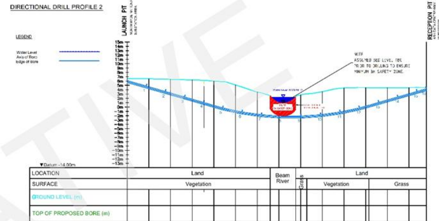
DIRECTIONAL DRILL PROFILE 2
